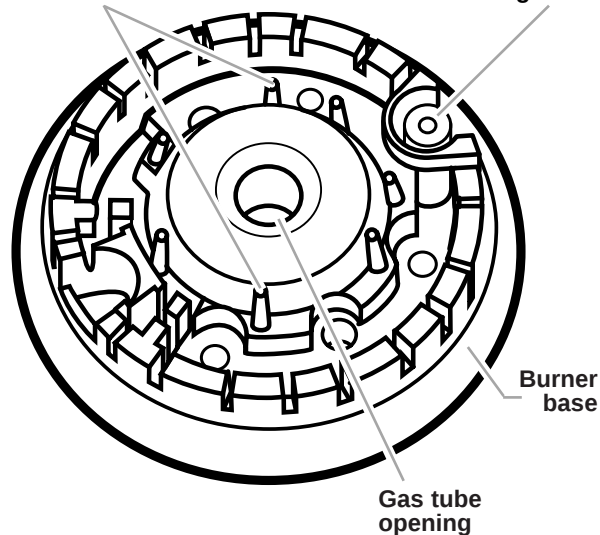
Ignitor
